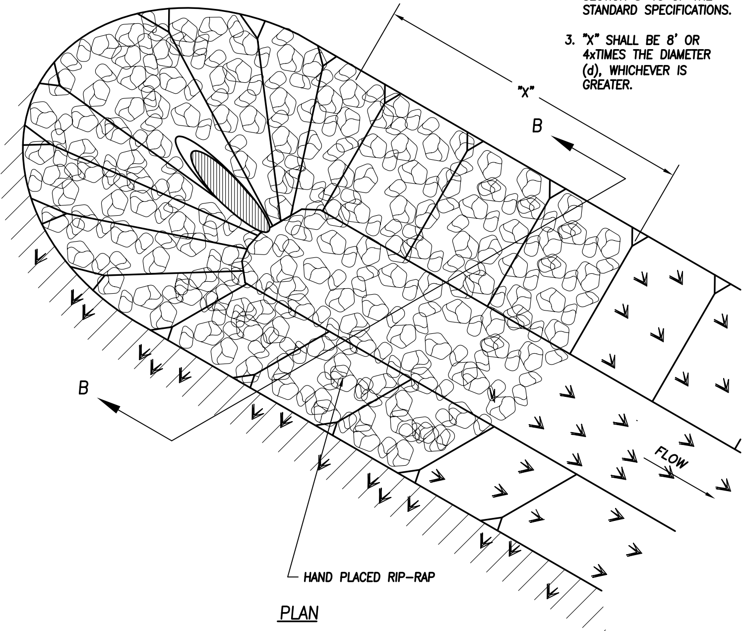
FLAT-BOTTOM DITCH RIP-RAP PLACEMENT DETAIL NTS
